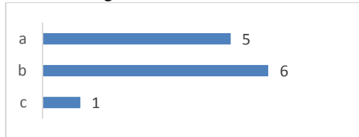
Fig. 6. Annotation forms
