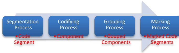
Fig. 2. Assessment cycle
