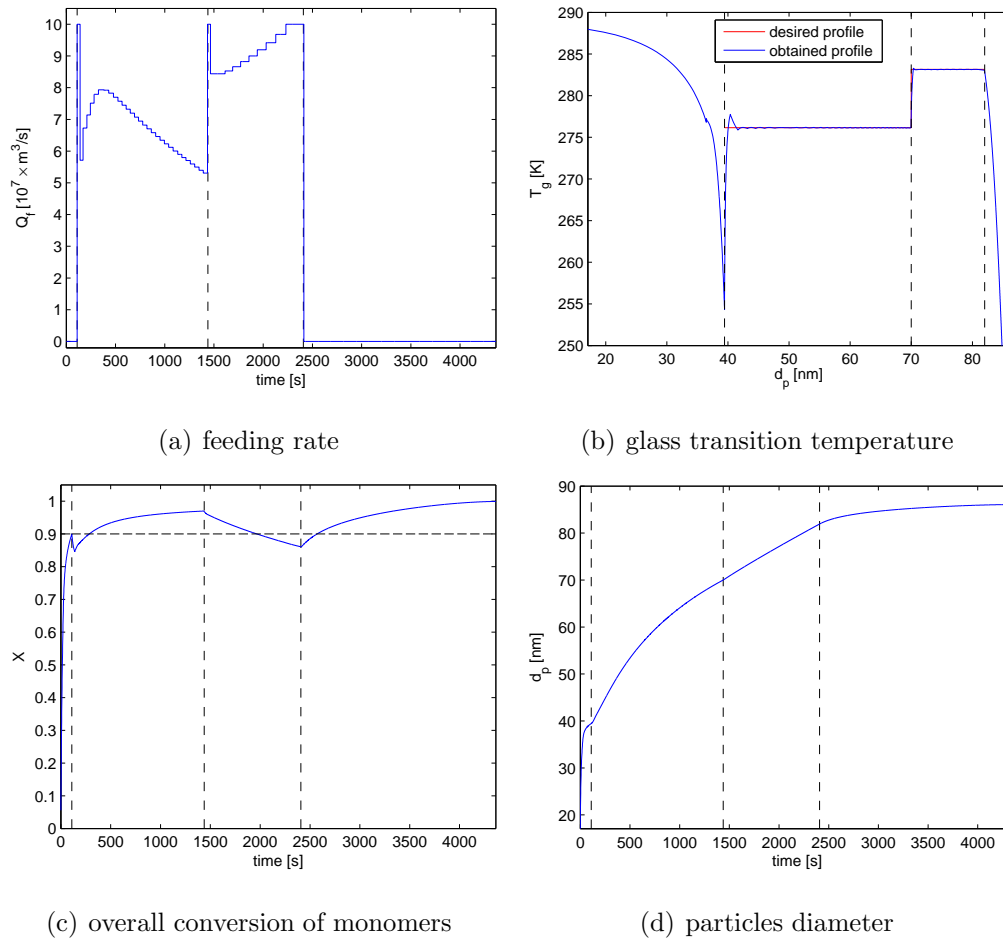
Figure 6: Optimal feeding policy and the corresponding state trajectories for scenario S5 (reaction at T=80^{\circ}\text{C} ).
