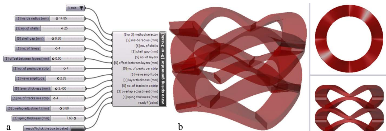
Figure 8 - Use of (a) the developed Grasshopper 3D cluster to generate (b) a closed mesh ready for G-code generation
