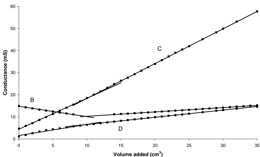
Figure 2. Conductometric titrations for cobalt gluconate.
