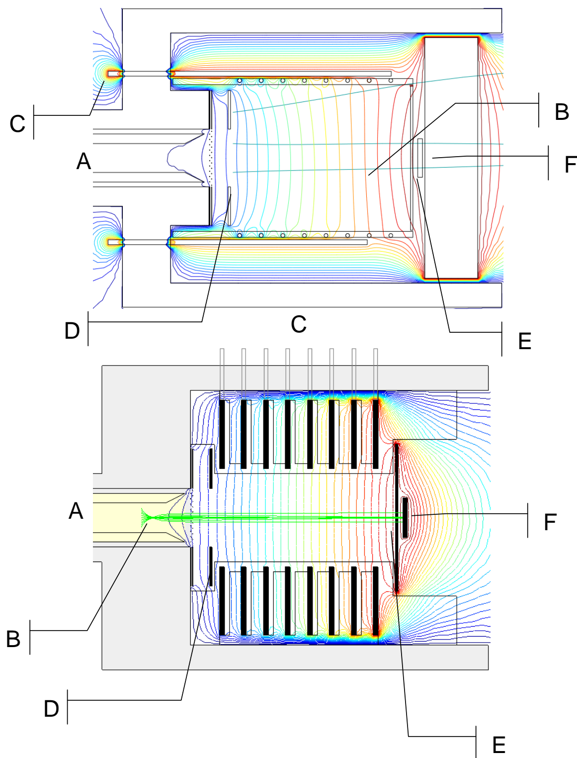
Figure 4 A comparison of the electric field models of the HiTMS (Top), and the polymer snap together tube (bottom). Key, A: inlet; B: ion trajectories; C: voltage supplies to field defining electrodes; D: shutter grid assembly; E: shield grid; F: Faraday detector.
