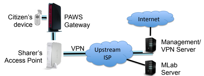
Figure 1: PAWS Architecture.
