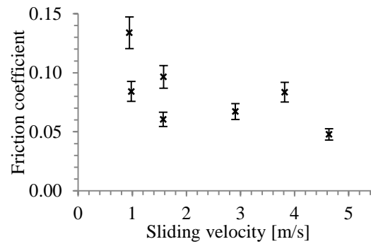
Figure 2 - Friction coefficient variation with sliding velocity for 1.2GPa contact pressure, 60°C bulk surface temperature for a lubricated contact
