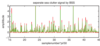
Fig. 6. Separated sea clutter signal by BSS, the red line is estimated signal and the green line is the original signal
