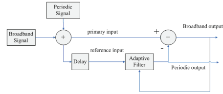
Fig. 2. Single sensor type of AIC processing structure
