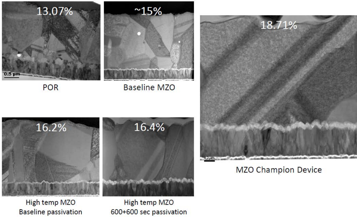
Supplementary Figure 1 | Cross-section HRTEM images of CdTe films showing the effect to larger CdTe grain size on device efficiency.
