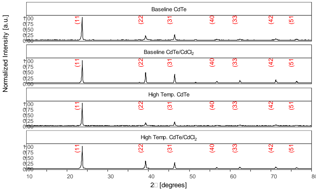
Figure 4 | XRD analysis of film orientation. XRD Peak intensities showing increased {111} orientation and less randomization of CdTe films sublimated at higher temperature on Mg 0.23 Zn 0.77 O buffer before and after CdCl 2 passivation treatment.
