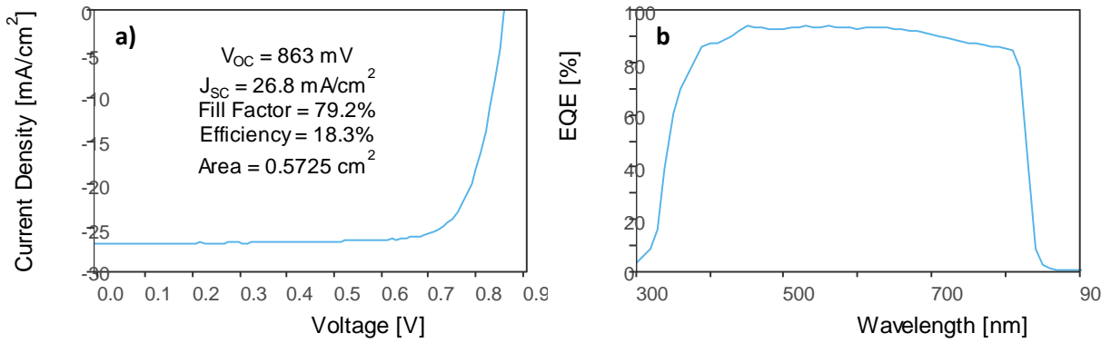
Figure 7 | ILX Lightwave certified results. (a) J-V Curve (b) and External quantum efficiency for device structure under investigation
