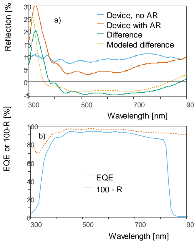
Figure 5 | AR Coating (a) Reflection vs wavelength comparing modeled against actual difference in reflection and (b) external quantum efficiency for AR coating used in this study.
