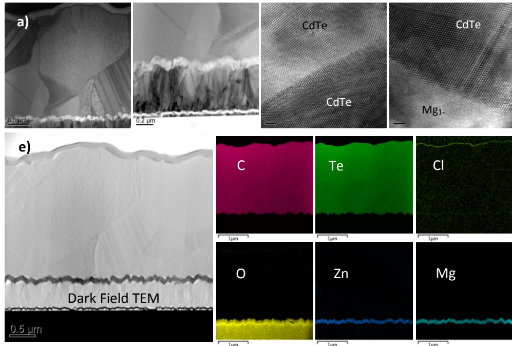
Figure 3 | Microscopic analysis. (a) TEM image TCO/Mg 0.23 Zn 0.77 O/CdTe/Te film stack (b) high magnification TEM image of TCO/ Mg 0.23 Zn 0.77 O and Mg 0.23 Zn 0.77 O/CdTe interface showing conformal coverage of Mg 0.23 Zn 0.77 O (c) HRTEM image of CdTe grain boundary showing no apparent signs of line or bulk defects (d) HRTEM image of Mg 0.23 Zn 0.77 O/CdTe interface showing abrupt interface with minimal intermixing (e) EDS elemental map of TCO/Mg 0.23 Zn 0.77 O/CdTe/Te film stack showing no diffusion of materials within detection limits.
