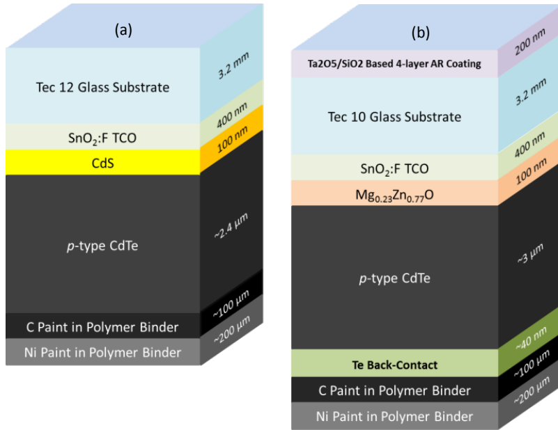
Figure 1 | Schematic of (a) CdS/CdTe baseline device (b) device with changes incorporated to achieve high efficiency (not to scale).
