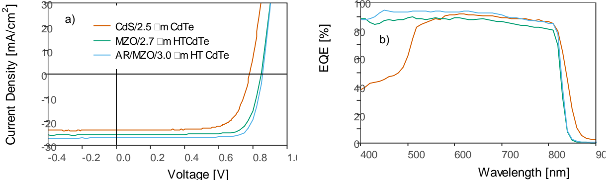
Figure 6 | J-V (a) and EQE (b) comparing performance of CdS/CdTe baseline device, MZO/CdTe high temperature (HT) device and high efficiency high temperature (HT) device with AR coating
