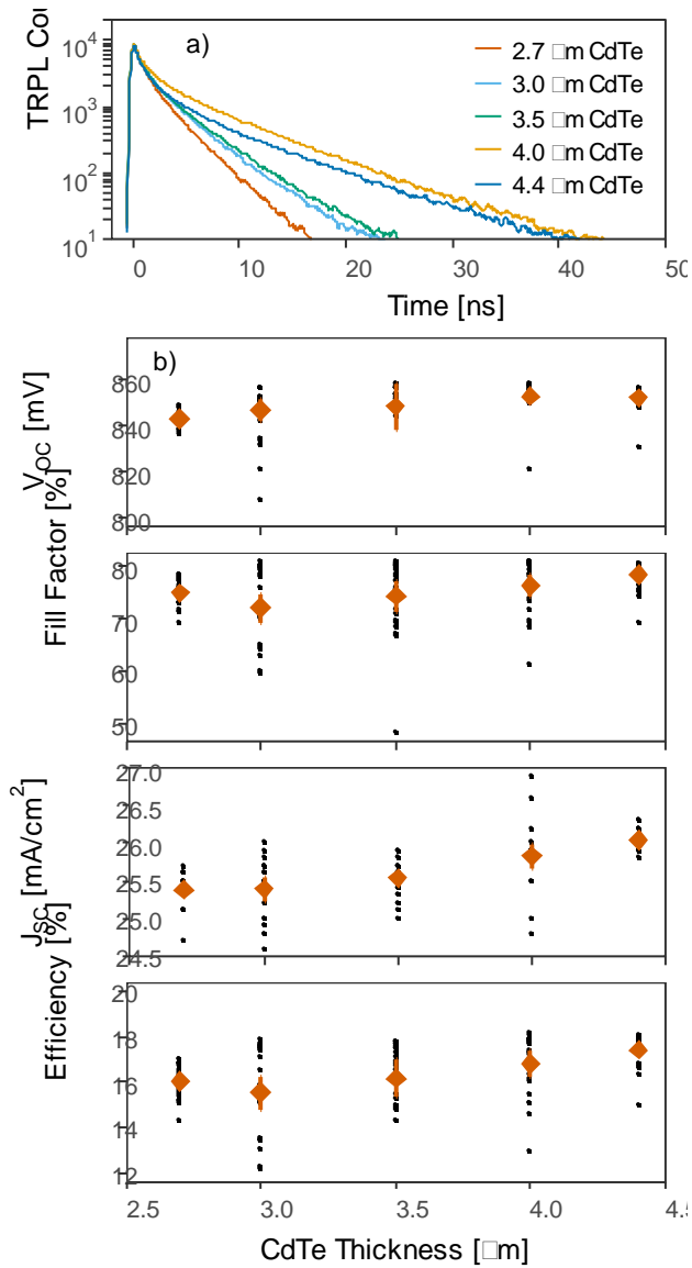
Figure 2 | Effect of varying absorber thickness (a) TRPL measurement showing improved carrier lifetime with increasing absorber thickness (b) performance parameters of devices with varying absorber thickness.
