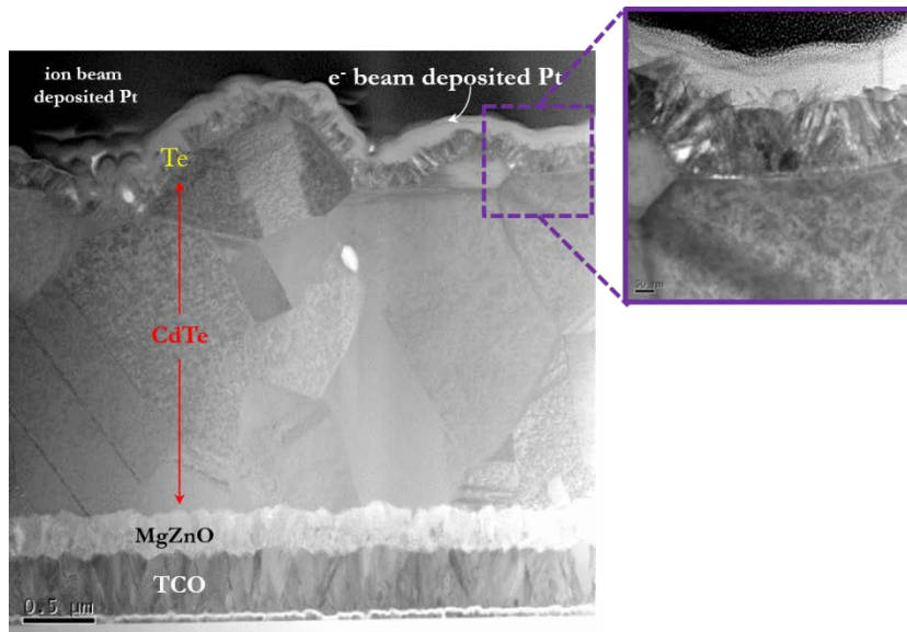
Supplementary Figure 2 | Cross-section HRTEM images of CdTe uniform coverage of Te on CdTe surface
