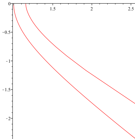
FIGURE 3. The resonances of Example 5.5 in the lower half plane are situated within the area between the two red curves.
