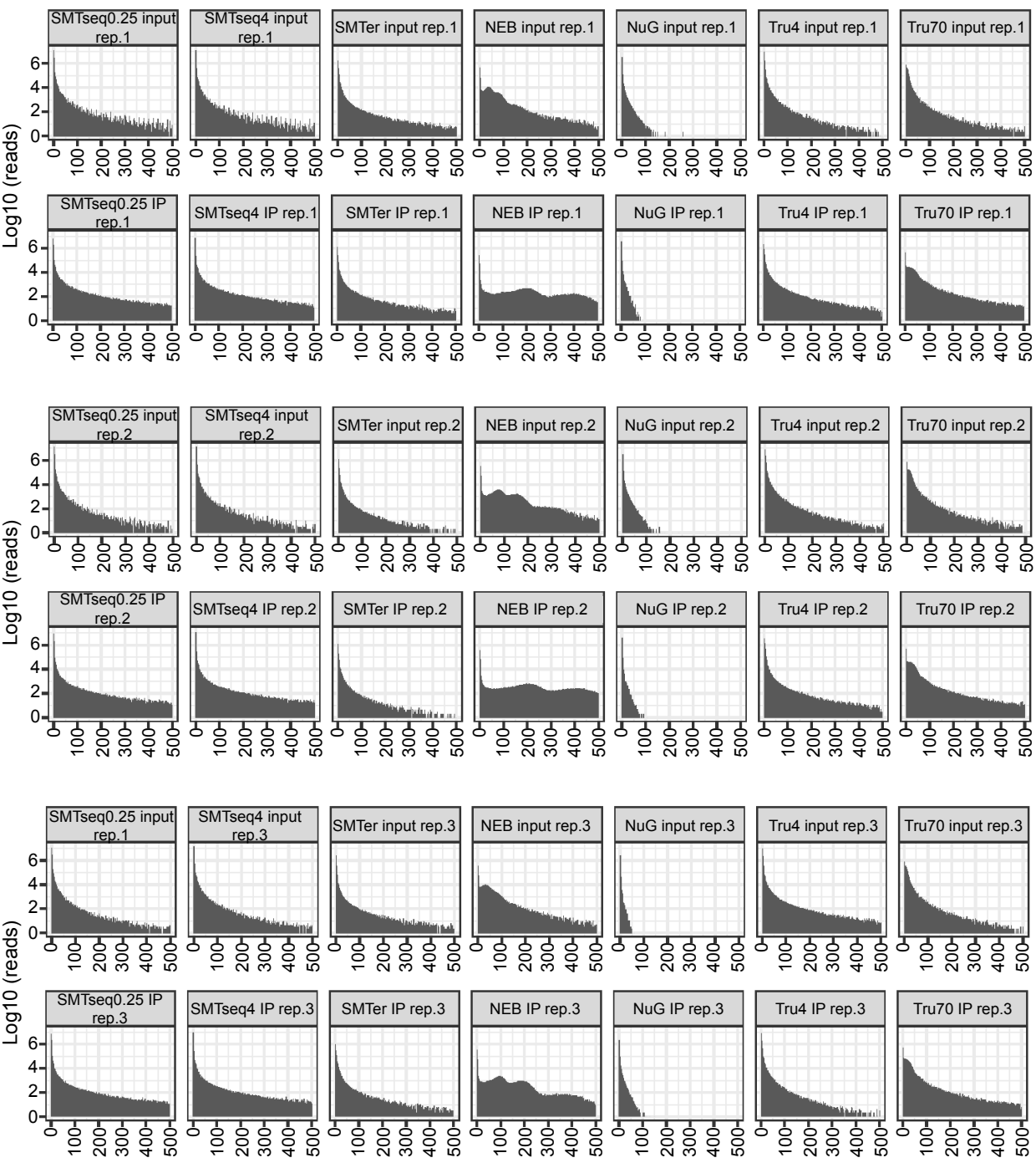
Fig. S2 Duplication rate of each library
