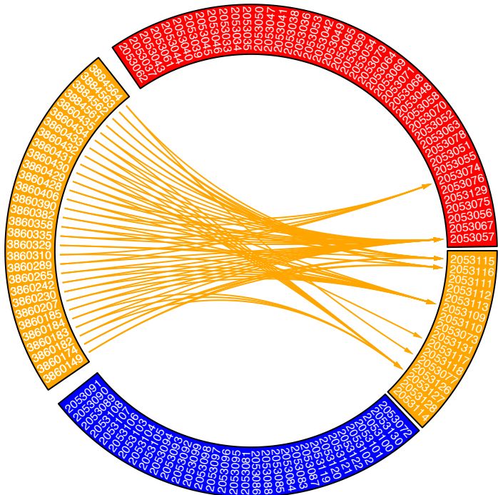
(B) Circular plots using the Manhattan distance
