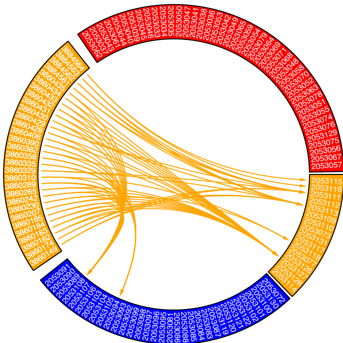
(A) Circular plots using the d_2^S dissimilarity
