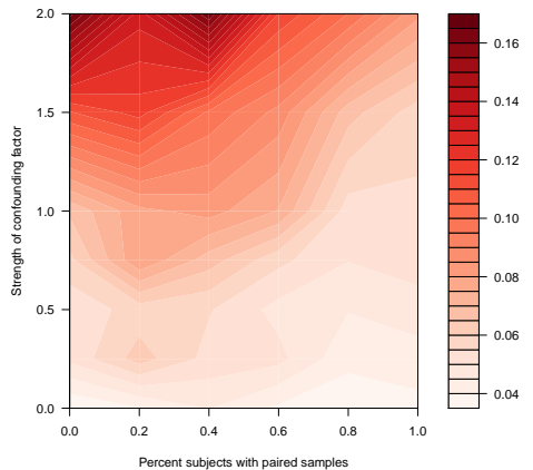
SD FDR with 50 total samples
