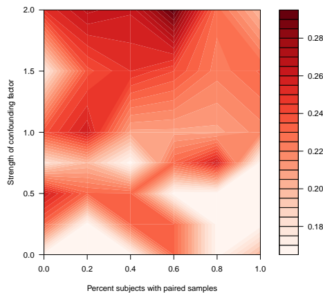
Range FDR with 100 total samples
