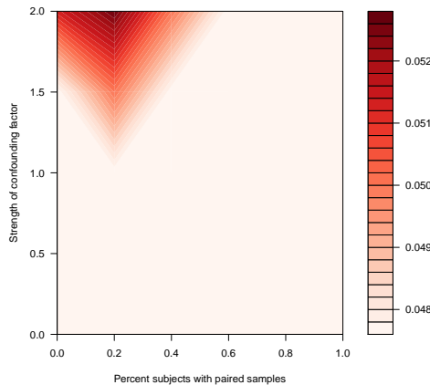
Median FDR with 200 total samples
