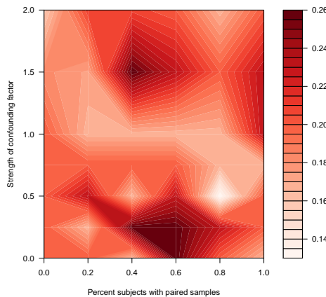
Range FDR with 200 total samples
