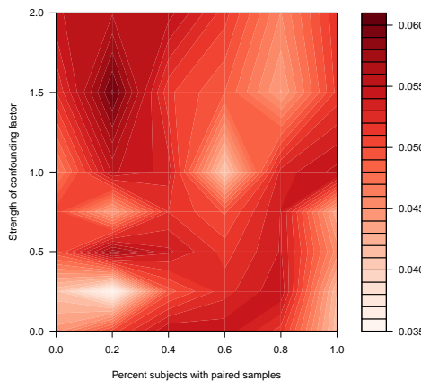
Ave. FDR with 500 total samples
