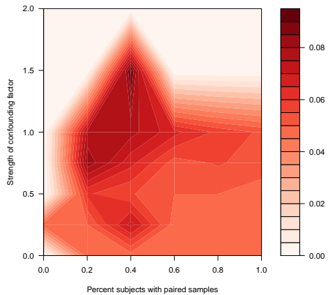
Median FDR with 50 total samples
