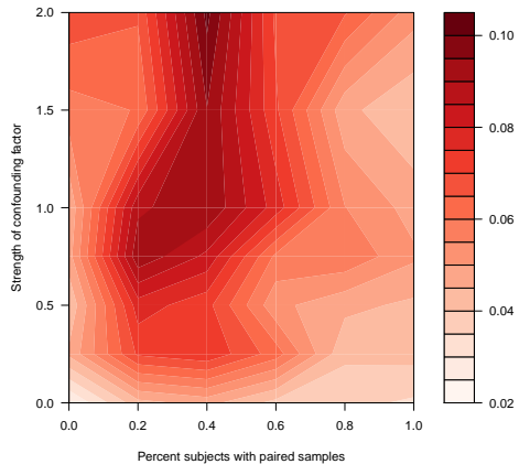
Ave. FDR with 50 total samples
