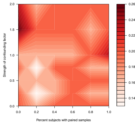
Range FDR with 500 total samples
