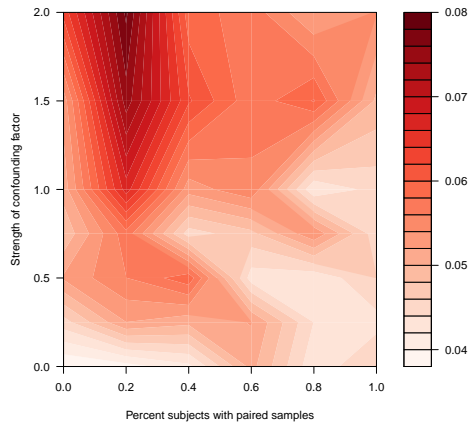
SD FDR with 100 total samples
