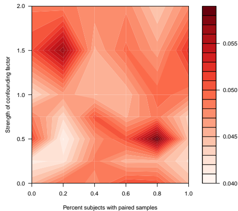
SD FDR with 500 total samples
