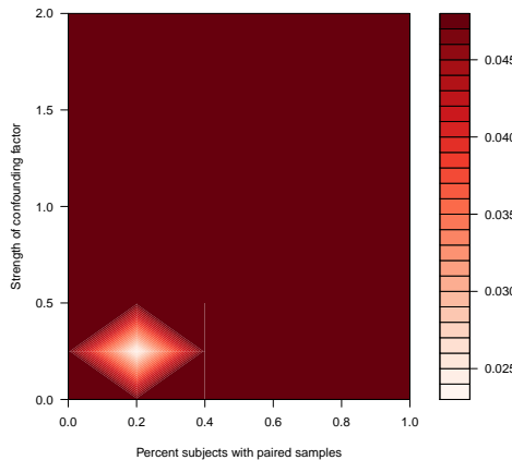
Median FDR with 500 total samples
