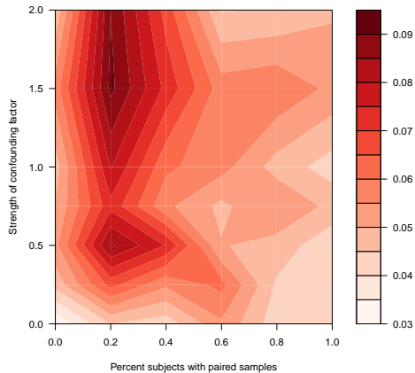
Ave. FDR with 100 total samples
