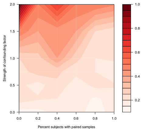
Range FDR with 50 total samples
