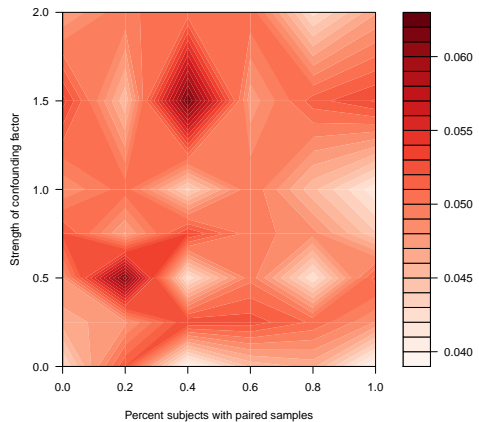
SD FDR with 200 total samples
