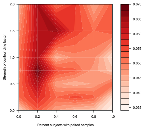
Ave. FDR with 200 total samples
