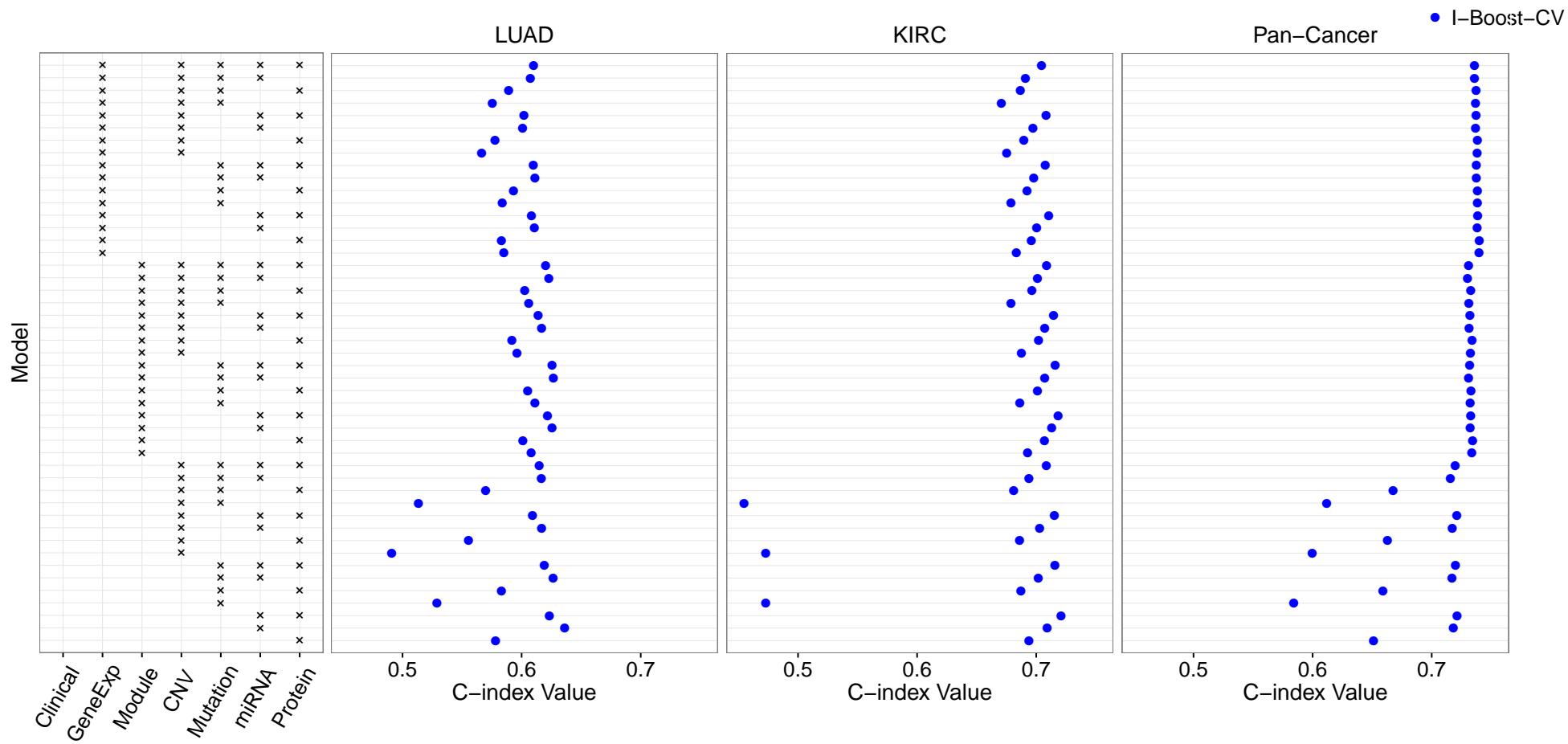
Fig. S1 Analysis results for the TCGA LUAD, KIRC, and pan-cancer data sets using I-Boost-CV. Each row represents a particular combination of data types used as predictors, as indicated by the box on the left. Each dot is an average C-index value obtained by performing I-Boost-CV on 30 training and testing data set pairs. See the caption of Fig. 1 for the abbreviations of the data types
