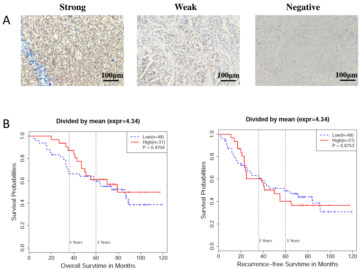
Figure S6. PLEKHM3 expression is not associated with survivals of ovarian cancer patients. (A) The protein expression of PLEKHM3 was measured by IHC analysis. 9 of 86 patients either failed to have a good IHC staining or did not acquired additional FFPE tissue blocks. (B) Kaplan–Meier survival analysis of PLEKHM3 expression in ovarian cancer patients. Differences in the survival risk between the two groups were assessed by the Mantel–Haenszel log-rank test.
