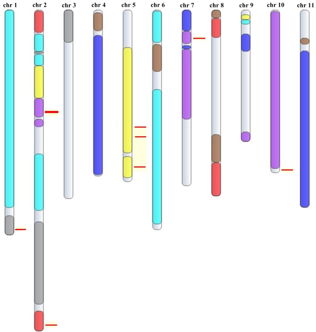
Supplementary Figure S1. Gene distribution of CcGH3 members on C. canephora chromosomes using the option "locus search" in the Coffe Genome Hub website. The colors within each chromosome indicate ancestral blocks corresponding to the 7 core eudicot chromosomes (DENOUEE et al., 2014). Red lines stand for the position of each CcGH3 over chromosomes. The most CcGH3 members are not presented in any chromosome, so they were allocated in chromosome 0 (not available). The genes are distributed as follow into each chromosome (chr): chr1: CcGH3.9 ; chr2: CcGH3.10 , CcGH3.11 and CcGH3.12 ; chr5: CcGH3.13 , CcGH3.14 and CcGH3.15 ; chr7: CcGH3.16 ; chr10: CcGH3.17 .
