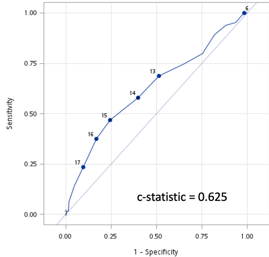
(b) Modified Adult Appendicitis Score
