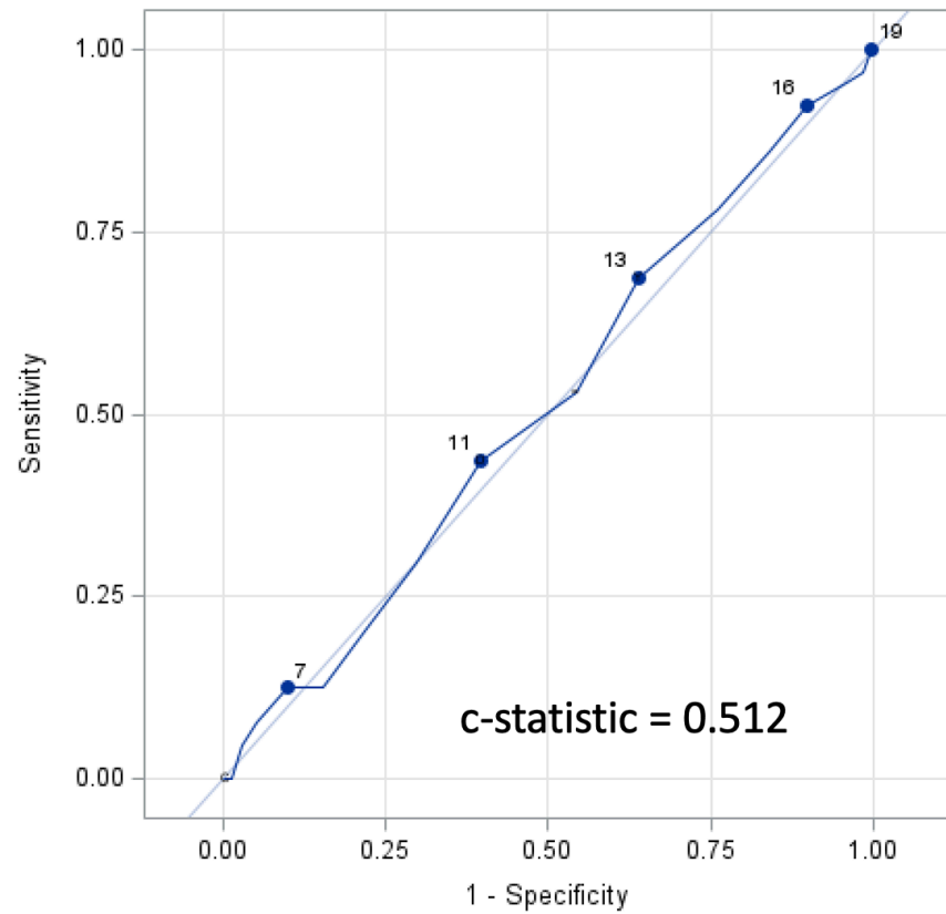
(a) Original Adult Appendicitis Score
