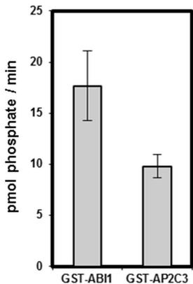
Figure S3. Activity of recombinant PP2Cs used in this study. Activity of 2 \mu\text{g} of each recombinant phosphatase was measured using the Serine/Threonine Phosphatase Assay System (Promega). The results were used for calculation of the amount of enzyme releasing 1 picomole of phosphate per minute (U) for each of the phosphatases. Error bars indicate SD ( n = 3 ).
