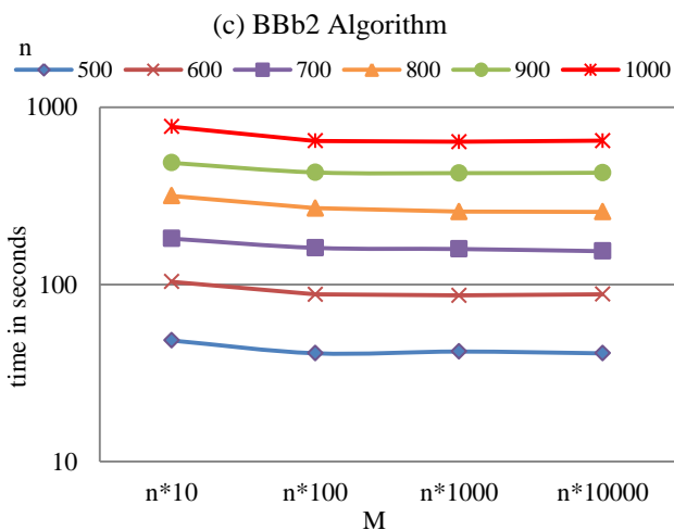
Figure F1: Running time of BBd, BBb, and BBb2 algorithms with different values of M.
