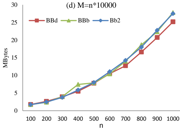
Figure F2: Memory consumed of BBd, BBb, and BBb2 algorithms on RD.
