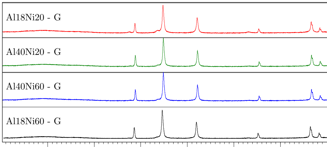
Figure 1: XRD graphs of the grinded samples, showing only Al and Ni phases.
