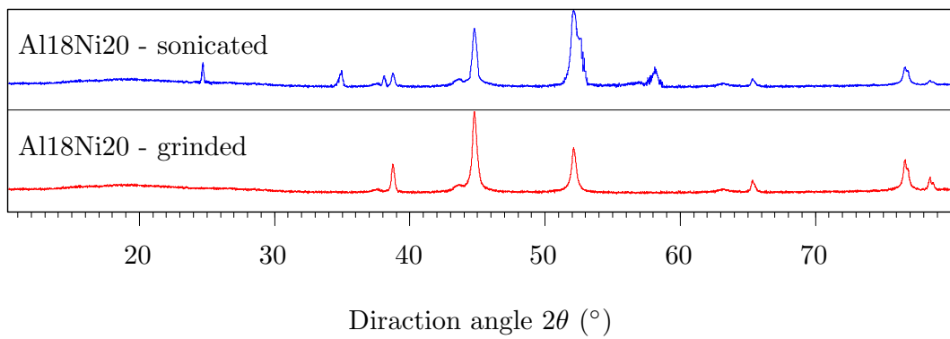
Figure 3: Comparison of XRD measurements of grinded and sonicated Al18Ni20 samples. The sonicated sample shows vast amounts of \text{Al}_2\text{O}_3 , while the grinded sample shows no oxidized phases.
