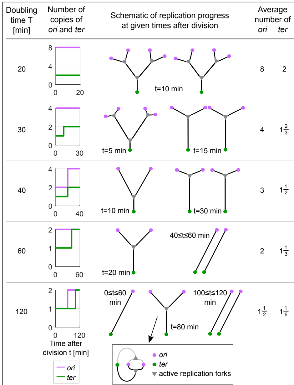
Figure S1: Genome replication based on the Cooper and Helmstetter's model [1, 3]. In the schematic of replication progress for simplicity only one half of a circular genome spanning ori and ter is shown (shown in black in the legend box).
