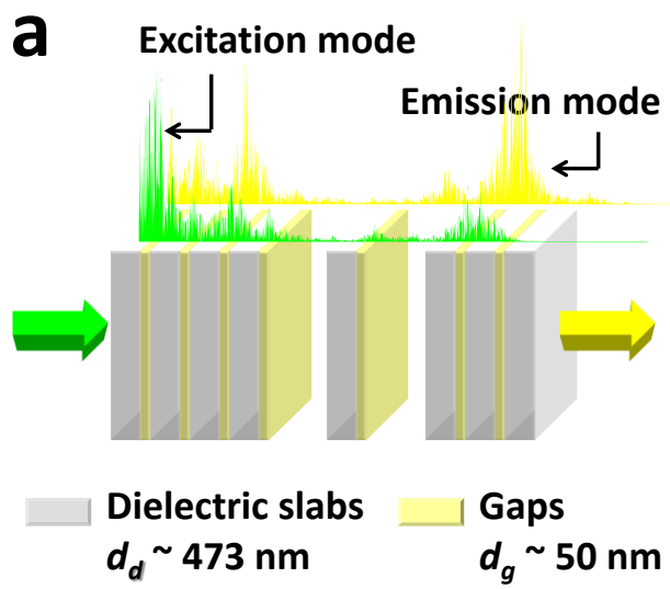
Fig. 1. (a). Schematic illustration of 1D multilayered nanostructures with alternating dielectric and gap (gain for lasing modes) layers. (b). Averaged transmission as a function of the number of dielectric layers.
