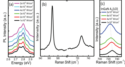
Fig. 2. (a) Photoluminescence spectra of InGaN/GaN MQWs under different excitation power density with an excitation wavelength of 325 nm, (b) and (c) Raman scattering spectra of InGaN/GaN MQWs with an excitation wavelength of 325 nm.
