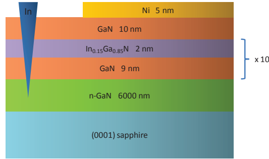
Fig. 1. The schematic structure of InGaN/GaN MQWs and Ni thin film
