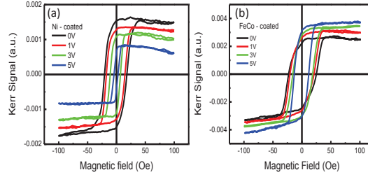
Fig. 3. (a) and (b). Hysteresis curves of Ni-coated and FeCo-coated InGaN/GaN MQWs by means of MOKE measurement with the applied magnetic field parallel to the plane of the sample under different external electric potentials.
