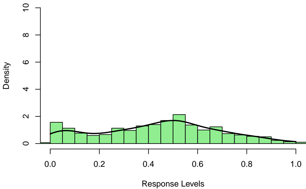
C) Responders and Non-responders
