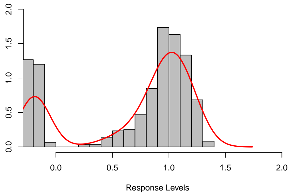
D) Bi-Directional Power Transform
