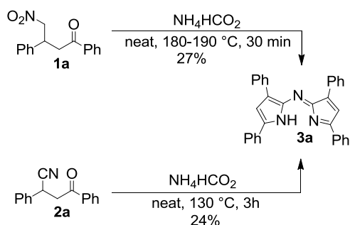
Scheme 1 Synthetic routes to azadipyrromethene developed by Rogers.
