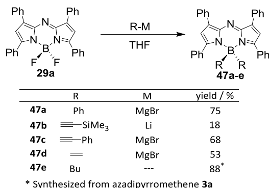
Scheme 21 Fluorine displacement with C-nucleophiles.
