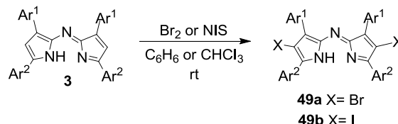
Scheme 23 Synthesis of dibromo- or diiodo-azadiarylmethanes.
