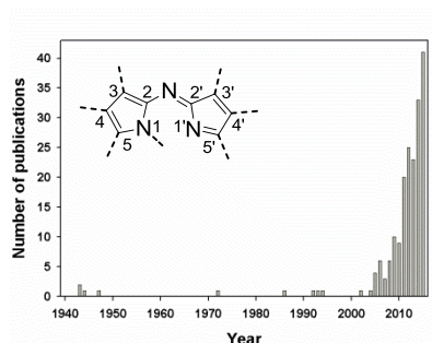
Fig. 1 Structural scaffold of azadipyrromethenes and yearly number of publications dealing with azadipyrromethenes according to SciFinder Scholar structure search (reviews not included) performed in January, 2016.
