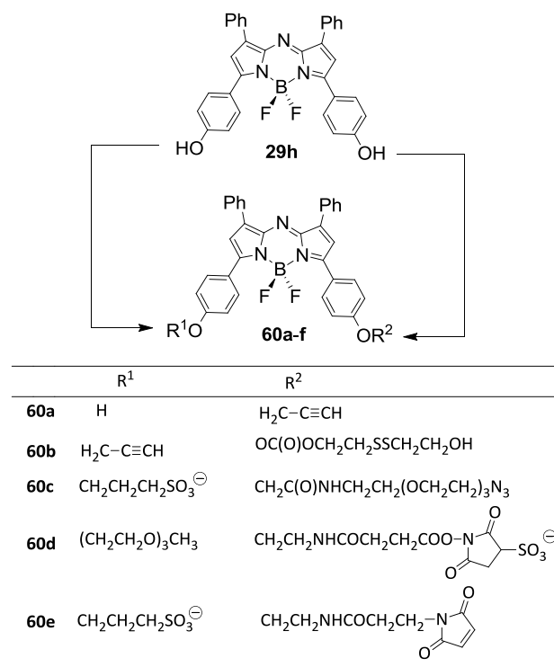
Scheme 31 Azadipyrromethene fluorochromes.
