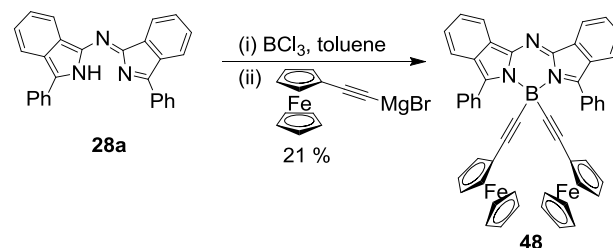
Scheme 22 Ferrocene-azadiarylmethane triad.
