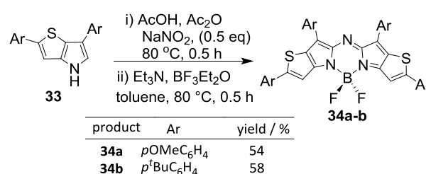
Scheme 14 \beta -Thiophene-fused BF 2 -azadipyrromethenes.
