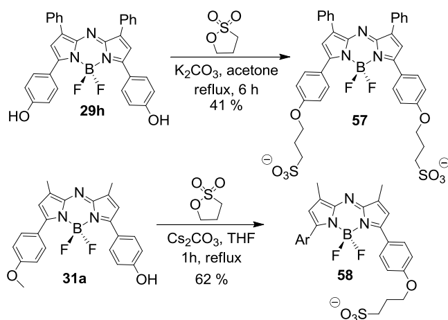
Scheme 29 Aqueous soluble derivatives.
