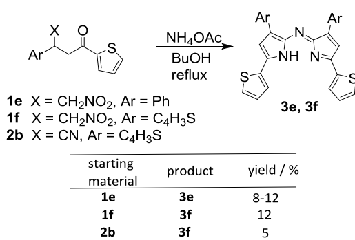
Scheme 5 Synthesis of thiophene substituted azadihydropyrimethenes.
