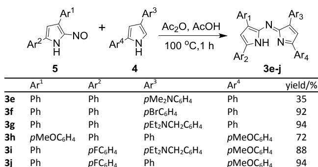
Scheme 7 Route to non-symmetric azadihydropyrimethenes.
