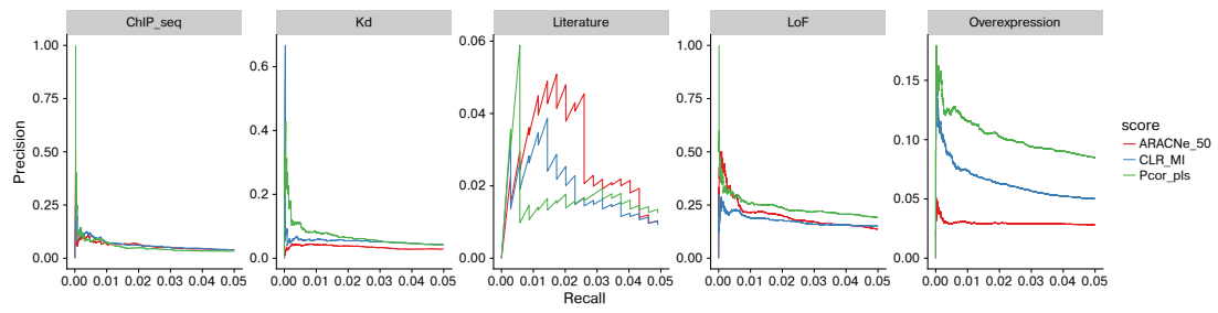
Supplementary Figure 2: Precision-Recall curves until a recall of 0.05 for the top performing algorithms on all gold standards.
