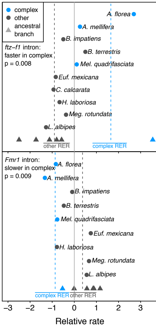
Figure S9. Two intronic NCARs associated with complex social behavior are key regulators of mushroom body neuronal remodeling ( ftz-f1 ; [23]) and development ( Fmr1 ; [24]). ftz-f1 shows accelerated rates of change on complex social branches relative to the remaining branches in the tree (relative rates test, p=0.008 ). Fmr1 shows significantly slower evolution on complex social branches (relative rates test, p=0.009 ).
