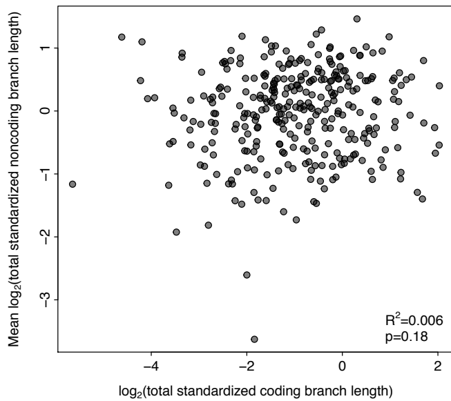
Figure S6. Log-transformed total branch length of coding sequences and proximal NCARs standardized to the branch lengths inferred from all a concatenation of all protein sequences. When multiple NCARs were associated with individual genes, mean standardized branch lengths were used.
