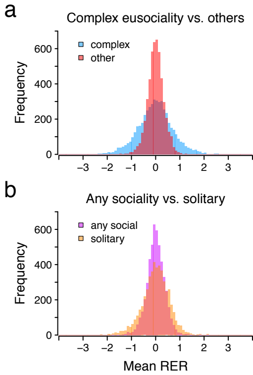
Figure S7. (a) Distribution of mean relative rates among taxa with complex sociality vs. others in all coding sequences. (b) Distribution of mean relative rates among taxa with any degree of sociality vs. strictly solitary taxa in all coding sequences.
