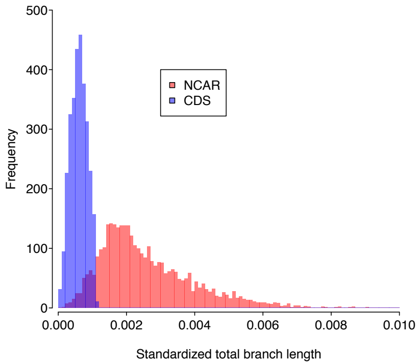
Figure S8. Distribution of total evolutionary change in all CDS's and NCARs analyzed. To make these measures comparable across loci and sequence classes, the standardized total evolutionary change was additionally divided by the number of bases in each locus.
