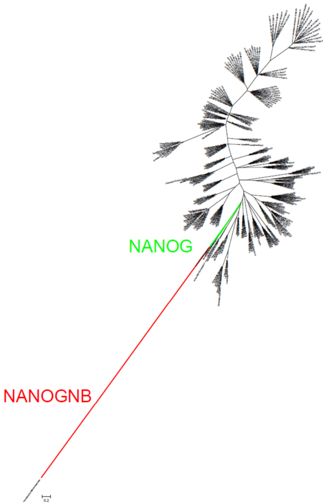
Supplementary Figure 1. Tree of all human, chicken, and zebrafish ANTP homeodomain sequences.
