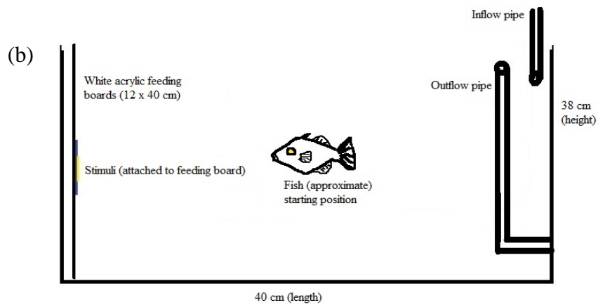
Supplementary Figure 1. Within-tank view of presenting tank-end (a). Note: the PVC hide was removed, and air pump was switched off during both training and experiments. Illustration of experimental aquaria (b) showing the approximate starting position of fish relative to presented stimuli.
