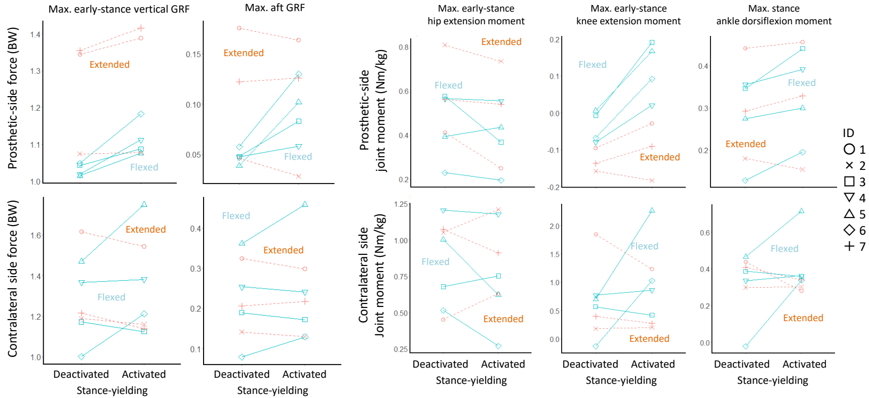
Supplementary Figure 2. Early-stance peak values for ground reaction force and joint moment. Solid lines indicate those who flexed the prosthetic knee during early stance (Flexed), and dashed lines indicate those who did not (Extended) in the Activated condition. BW: body weight
