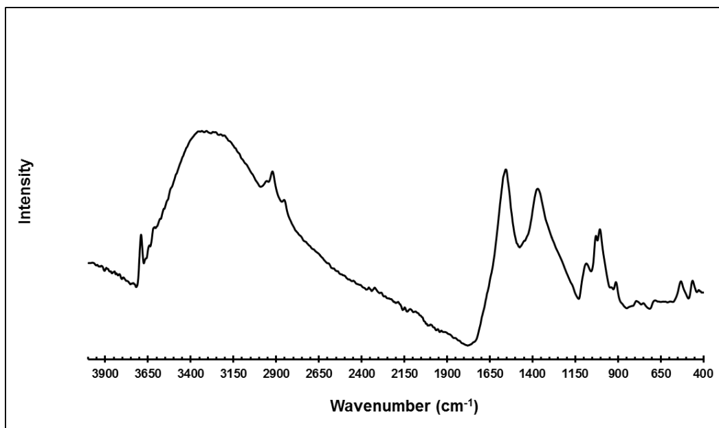
Supplemental Material Figure 2. IR spectrum of humic acid using the ATR technique
