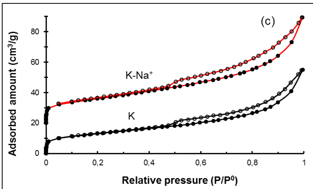
Supplemental Material Figure 1. N 2 adsorption–desorption isotherms of (a) Y-Na + and Y, (b) D-Na + and D, (c) K-Na + and K.
