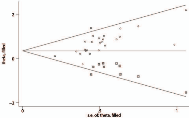
B Filled funnel plot with pseudo 95% confidence limits
