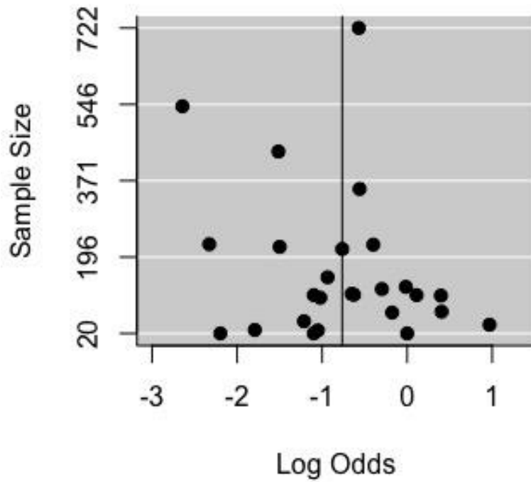
Figure 4. Funnel plot for the category of anxiety disorders
