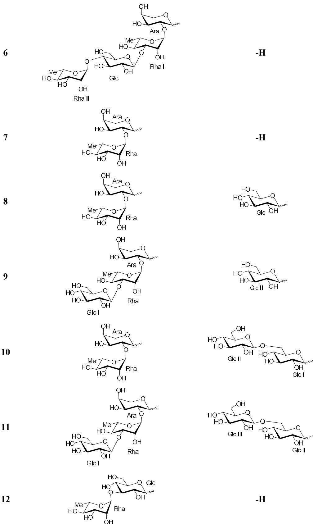
The structures of compounds 1-13 from Cephalaria tuteliana
