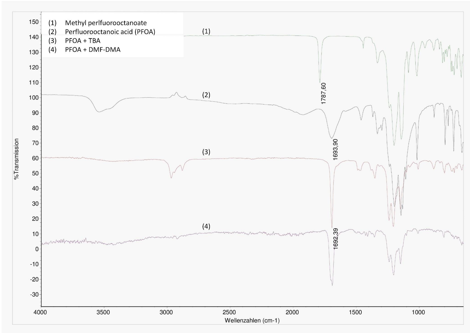
Figure 1 FTIR spectrum of PFOA, PFOA methy ester and reaction products of PFOA with tetrabutylammonium hydroxide and DMF-DMA
