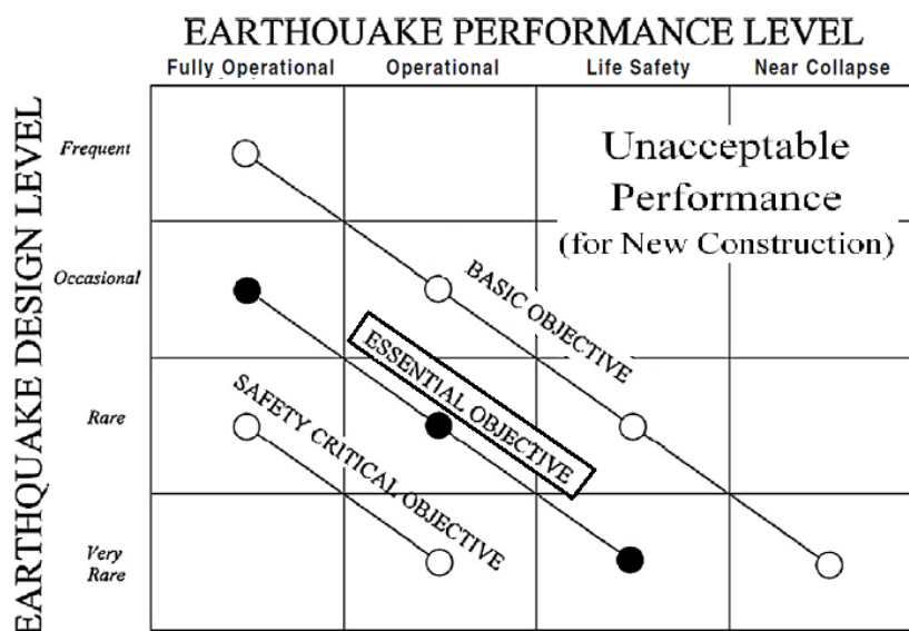
Figure 1- Performance-based seismic design objectives, adopted from [9]
