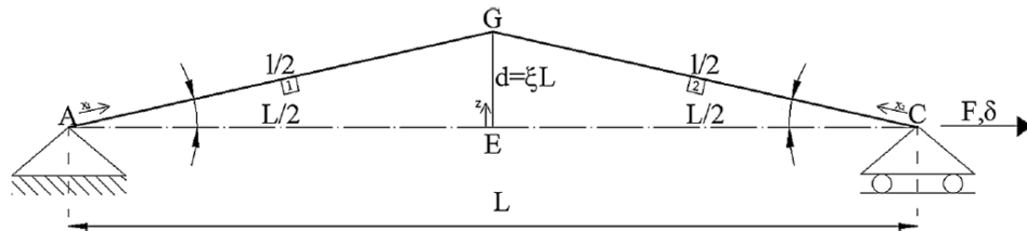
Figure 2- The geometric configuration of the studied device [8]
