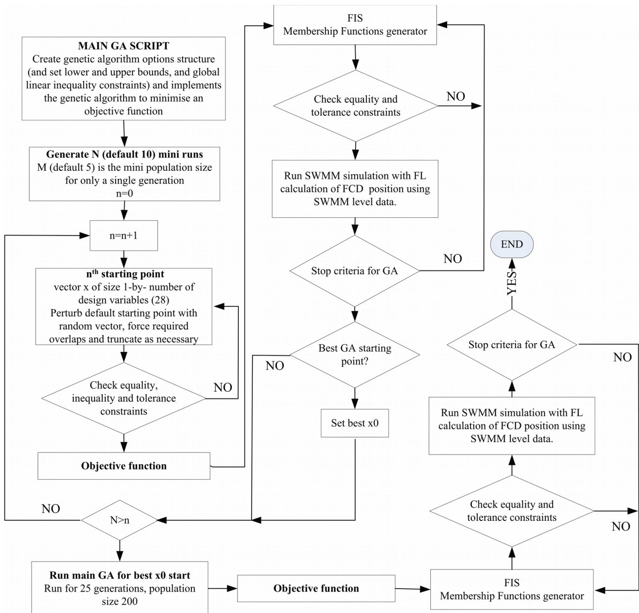
Figure 2. Flow diagram for GA optimisation module
