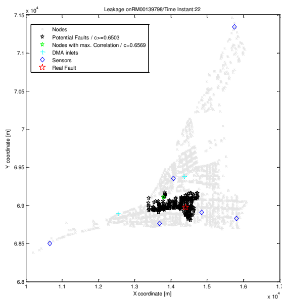
Figure 9: Performance of leak localization method (September 30th)
