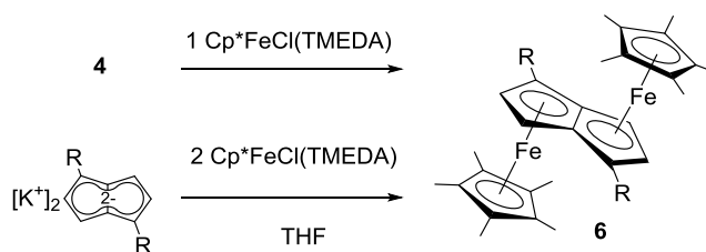
Scheme 7. Synthetic routes to 6 . R = Si i Pr 3 .
