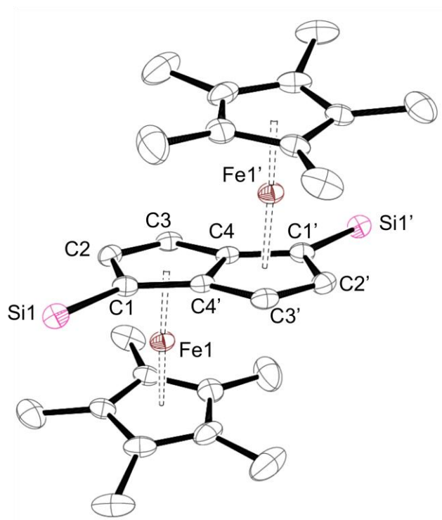
Fig. 7. Displacement ellipsoid plot (50% probability) of 6 . Hydrogen atoms and 1 Pr groups omitted for clarity. Primed atoms are generated by symmetry.
