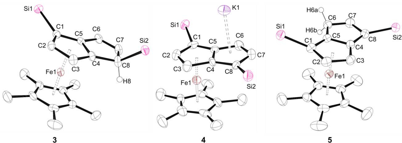
Fig. 5. Displacement ellipsoid plots (50% probability) of 3 , 4 and 5 . Hydrogen atoms (except allylic H's) and i Pr groups omitted for clarity.
