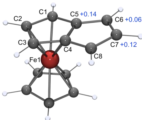
Fig. 10. Ball and stick diagram of calculated structure of [CpFe( \eta^5 -Pn)] - constructed from coordinates published by Saillard et al. [37] Labelling system for the Pn ligand shown in black and net charges on C atoms in blue.
