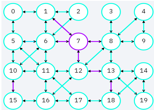
Figure 8: Connectivity map of ibmq-20-tokyo, qubits and links with high error rate are mark as purple
