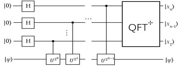
Figure 9: Quantum Phase Estimation circuit based on inverse QFT
