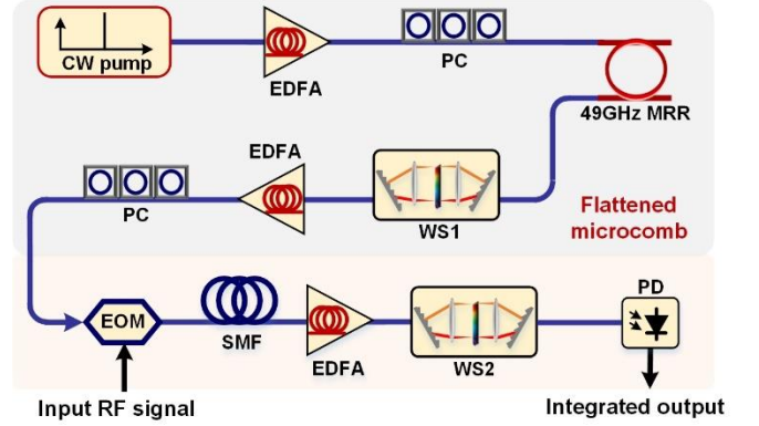
Fig. 2. Experimental setup of the photonic RF integrator based on a microcomb source. EDFA: erbium-doped fibre amplifier. PC: polarization controller. MRR: micro-ring resonator. WS: WaveShaper. EOM: Mach-Zehnder modulator. SMF: single mode fibre. PD: photodetector.
