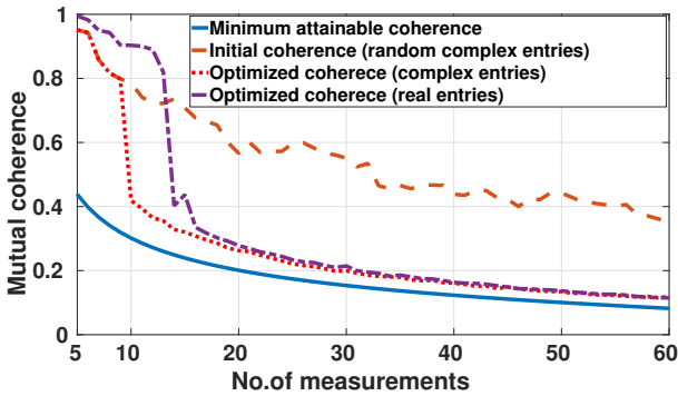
Fig. 1. Mutual coherence values for M \times 100 matrices for random, optimized, and real sensing matrices. The amplitude and phase of every matrix element has been quantized to 6 bits each (for the complex entries).
