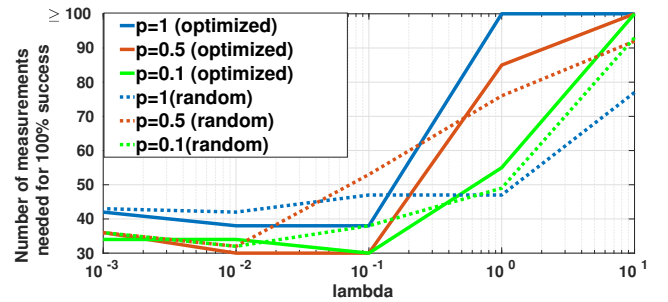
Fig. 2. Performance of IRL1 on a 100 element linear array for different values of the hyperparameter, \lambda for the case of (complex) random and optimized sensing matrices. The number of faults and SNR are fixed at 10 and 20 dB, respectively.
