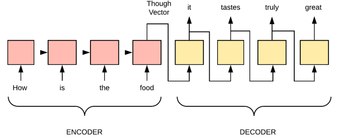
Fig. 1. Seq2Seq Model
