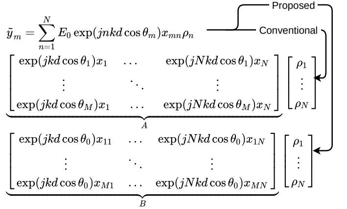
Fig. 2. A mathematical counterpart to the schematic in Fig. 1, showing the difference between the conventional and proposed method to generate a set of measurements. In the former, measurement locations \theta_i are varied, keeping element excitations constant. In the latter, the measurement location is kept constant, while element excitations x_{ij} are varied. Due to the lower mutual coherence obtainable from matrix B , the proposed method gives high success in fault diagnosis. For the sake of illustration, we have set E_n(\theta) = E_0 , a constant, in (1).
