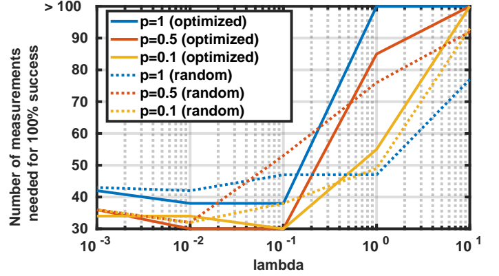
Fig. 4. Performance of IRL1 on a 100 element linear array for different values of the hyperparameter, \lambda for the case of (complex) random and optimized sensing matrices. The number of faults and SNR are fixed at 10 and 20 dB, respectively.
