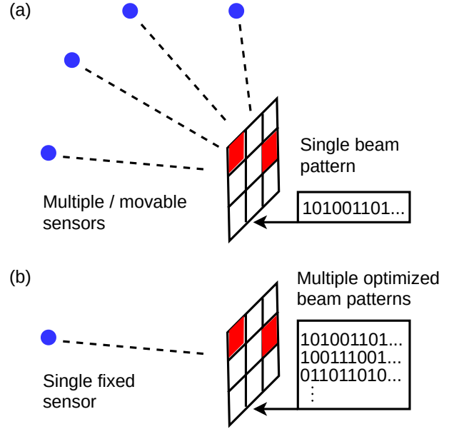
Fig. 1. Contrast between (a) conventional, and (b) the proposed method for fault detection. A sample 3 \times 3 phased array is shown by means of a grid, with the filled tiles indicating a faulty element. The filled circles indicate a field measurement sensor, the dashed lines indicate wave propagation between the array and the sensor(s), and a single line of a binary pattern indicates the inputs to the amplitude and phase control of the phased array. For the proposed method, the input signals are optimized in order to minimize the mutual coherence of the sensing matrix. Fig. 2 shows a mathematical depiction of the same idea.
