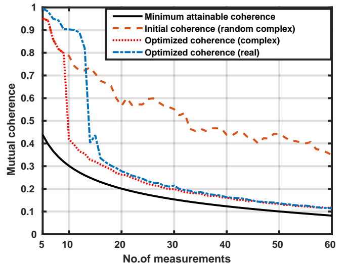
Fig. 3. Mutual coherence values for M \times 100 matrices for random, optimized, and real sensing matrices. The amplitude and phase of every matrix element has been quantized to 6 bits each in the case of complex measurements, whereas this quantization is to 6 bits amplitude and 1 bit phase (i.e. a \pm sign), in the case of real measurements.
