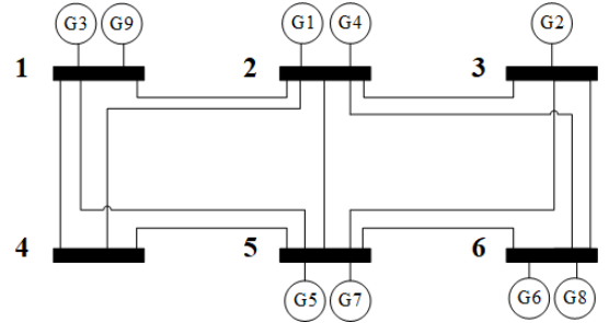
Figure 2: 6-bus system
