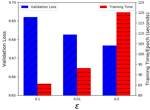
Figure 7: Effects of adjacency matrix threshold values in Spatiotemporal GCRNN model. When \epsilon decreases from 0.1 to 0.0, the Validation Loss decreases but the Training Time also goes up.
