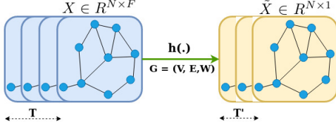
Figure 2: An air pollution forecasting task is constructed as a graph-based problem. T is the number of historical graph signals, T^\theta is the number of future prediction graph signals. X \in \mathbb{R}^{N \times F} is an input graph signal, \tilde{X} \in \mathbb{R}^{N \times 1} is an output signal, h(\cdot) is the learned function given the graph G .
