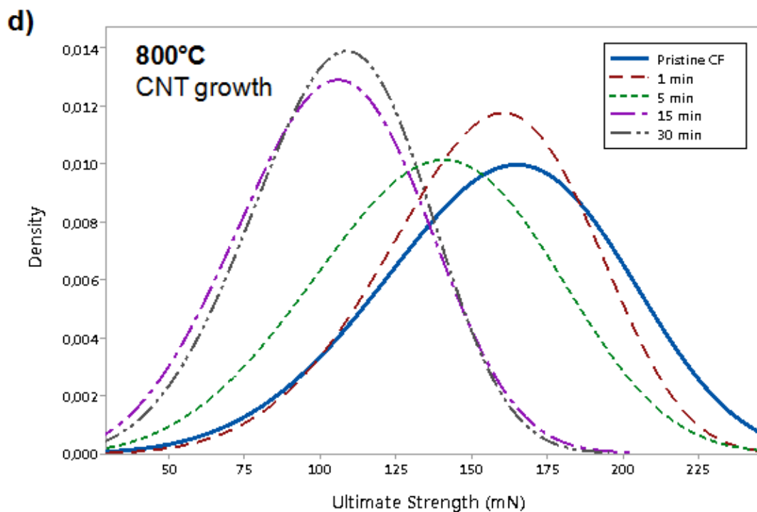
Figure 1: 2-Parameters Weibull Distribution for single-filament tensile strength tests. a) dependence on treatment time at 650°C under Ar atmosphere; b) idem at 800°C; c) dependence on treatment time at 650°C under CNT growth atmosphere; d) idem at 800°C.
