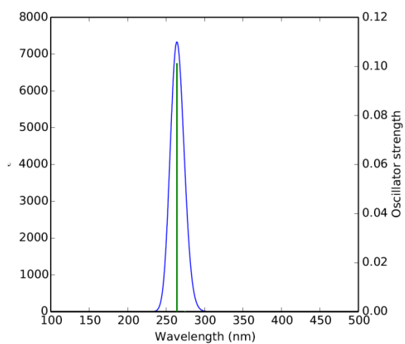
Fig.S2.5 UV spectrum of CA
