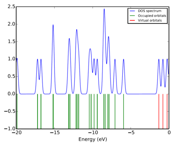
Fig.S1.9 DOS plot of BA
