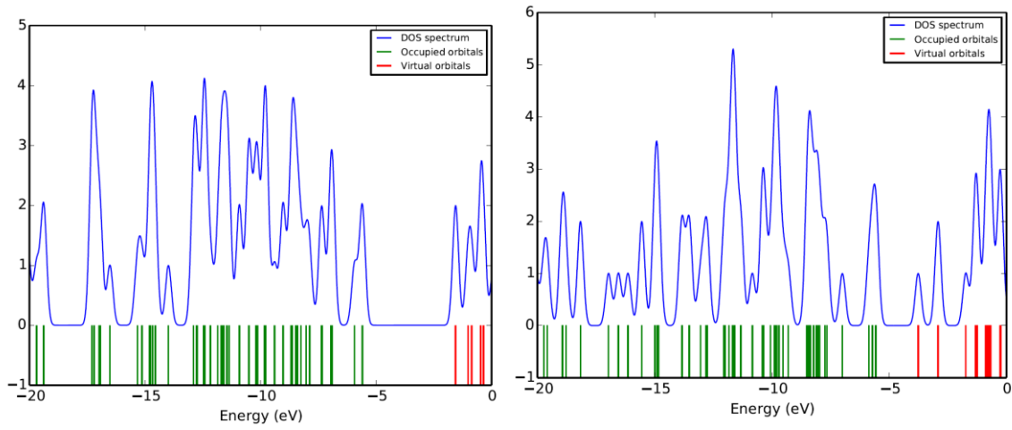
Fig.S1.11 DOS plots of AlN-BA and AlP-BA
