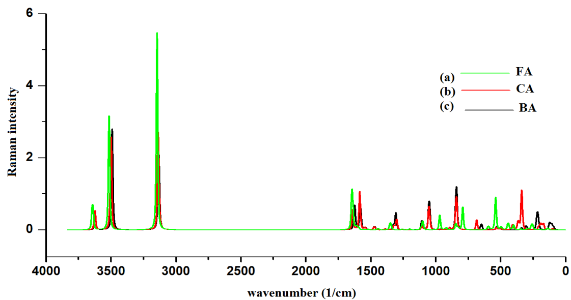
Fig.S3 Raman spectrum (DFT) of (a) FA (b) CA (c) BA
