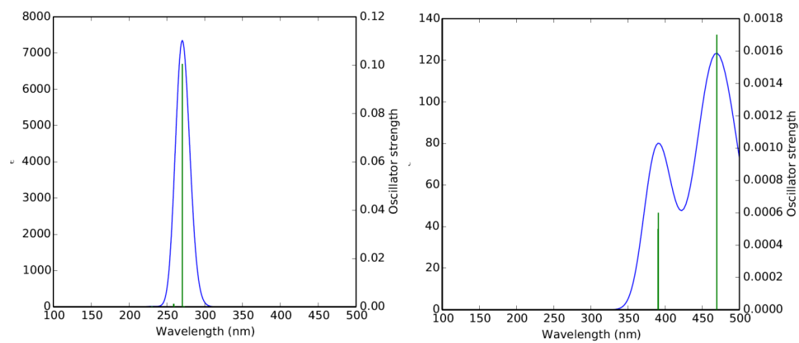
Fig.S2.9 UV spectrum of BA
