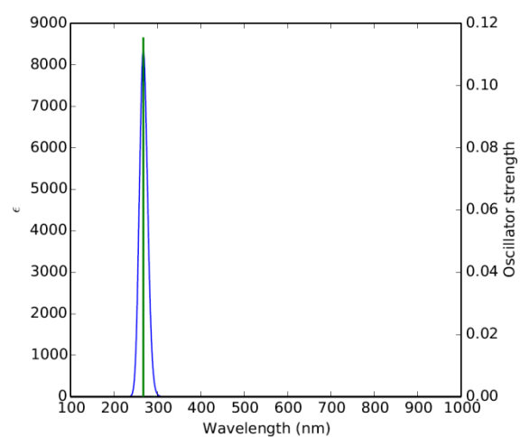
Fig.S2.9 UV spectrum of BA
