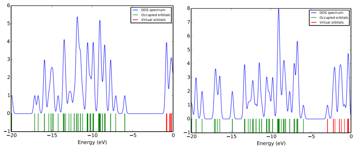
Fig.S1.9 DOS plot of BA
