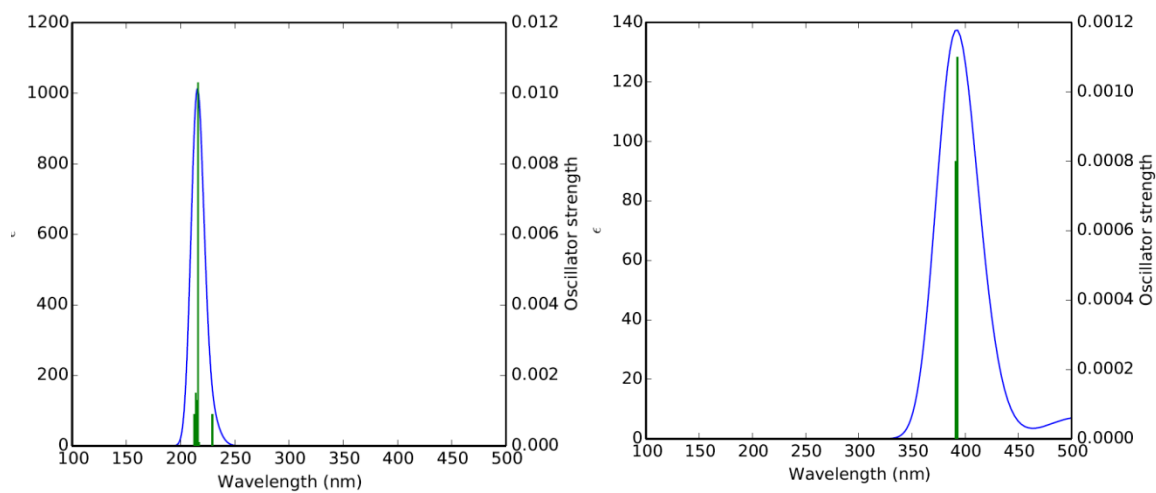
Fig.S2.5 UV spectrum of CA
