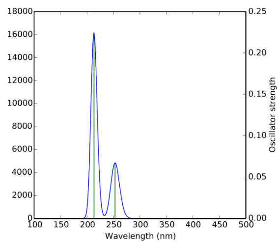
Fig.S2.1 UV spectrum of FA
