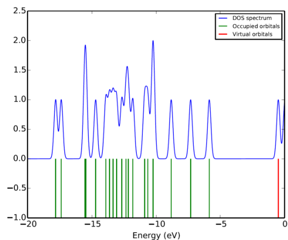
Fig.S1.1. DOS plot of FA
