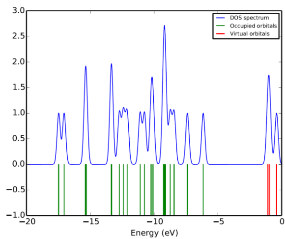
Fig.S1.5 DOS plot of CA
