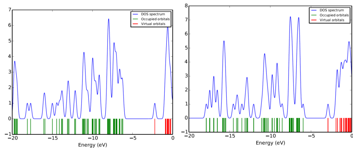
Fig.S1.3 DOS plots of AlN-FA and AIP-FA
