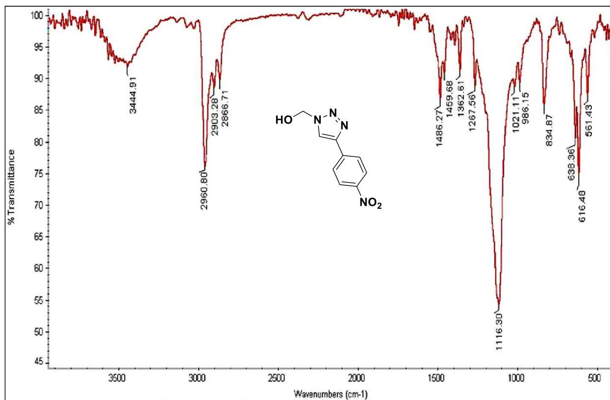
Fig. S16 FT-IR of (4-(4-nitrophenyl)-1H-1,2,3-triazol-1-yl)methanol ( 6g , Table 3, Entry 15)
