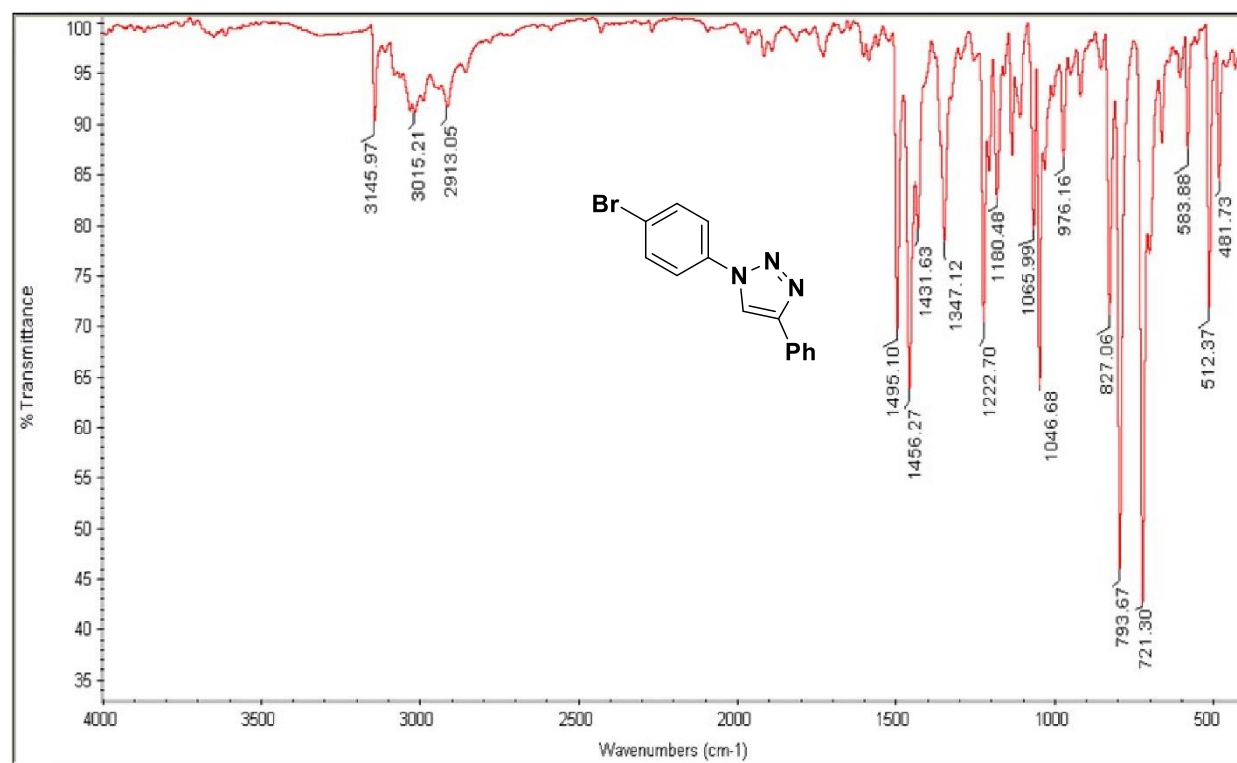
Fig. S15 FT-IR of 1-(4-bromophenyl)-4-phenyl-1H-1,2,3-triazole ( 6c , Table 3, Entry 11)
