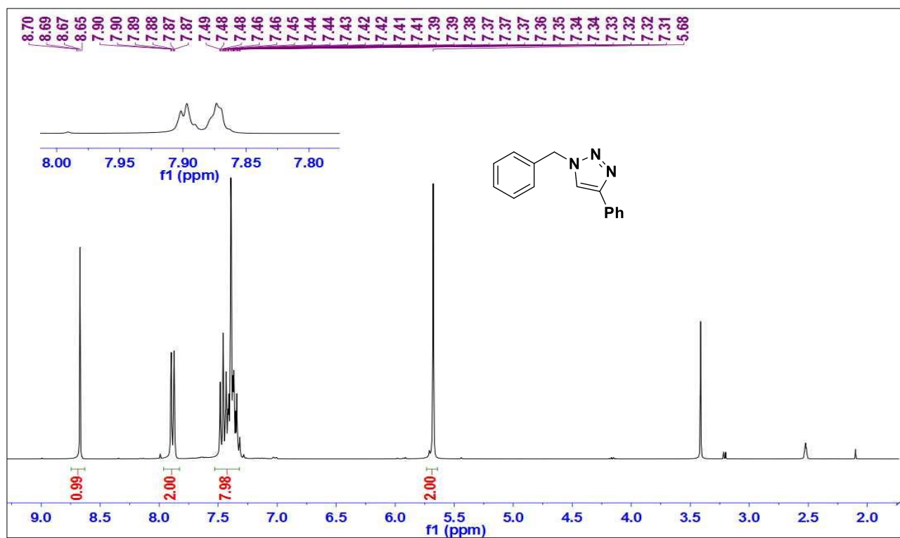
Fig. S4 ^1\text{H} -NMR of 1-Benzyl-4-phenyl-1H-1,2,3-triazole ( 5a , 5b and 5c , Table 3, Entries 1-3)
