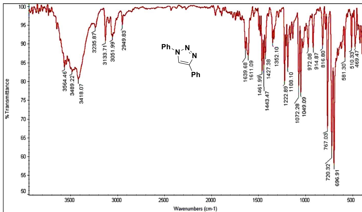
Fig. S13 FT-IR of 1,4-diphenyl-1 H -1,2,3-triazole ( 6a , Table 3, Entry 9)
