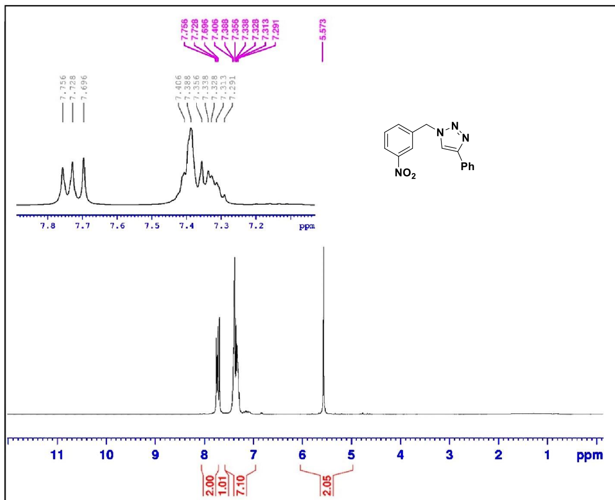
Fig. S12 ^1\text{H} -NMR of 1-(3-nitrobenzyl)-4-phenyl-1H-1,2,3-triazole ( 5h , Table 3, Entry 8)
