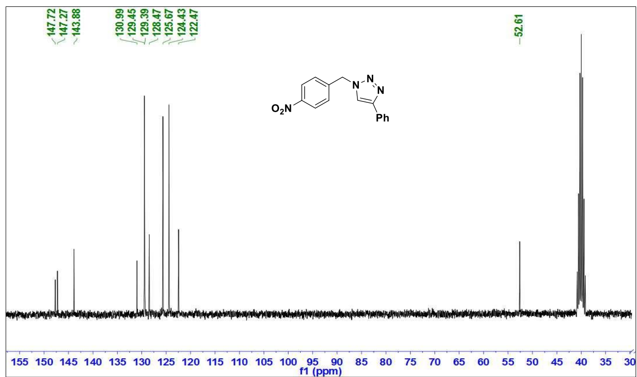
Fig. S10 ^{13}\text{C} -NMR of 1-(4-nitrobenzyl)-4-phenyl-1H-1,2,3-triazole (5f, Table 3, Entry 6)
