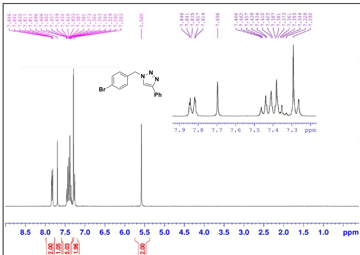
Fig. S11 1 H-NMR of 1-(4-bromobenzyl)-4-phenyl-1H-1,2,3-triazole (5g, Table 3, Entry 7)
