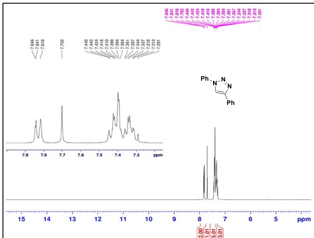
Fig. S14 1 H-NMR of 1,4-diphenyl-1 H -1,2,3-triazole ( 6a , Table 3, Entry 9)
