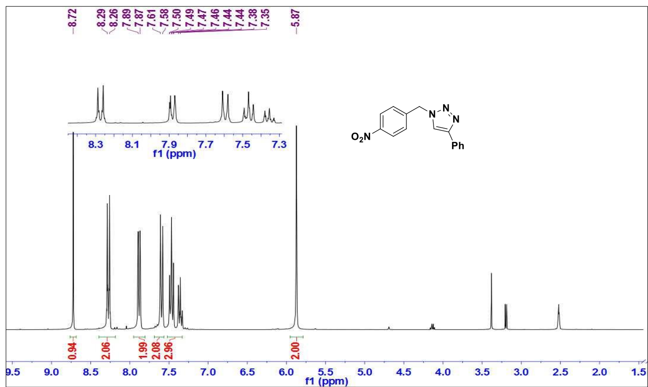
Fig. S9 ^1\text{H} -NMR of 1-(4-nitrobenzyl)-4-phenyl-1H-1,2,3-triazole ( 5f , Table 3, Entry 6)
