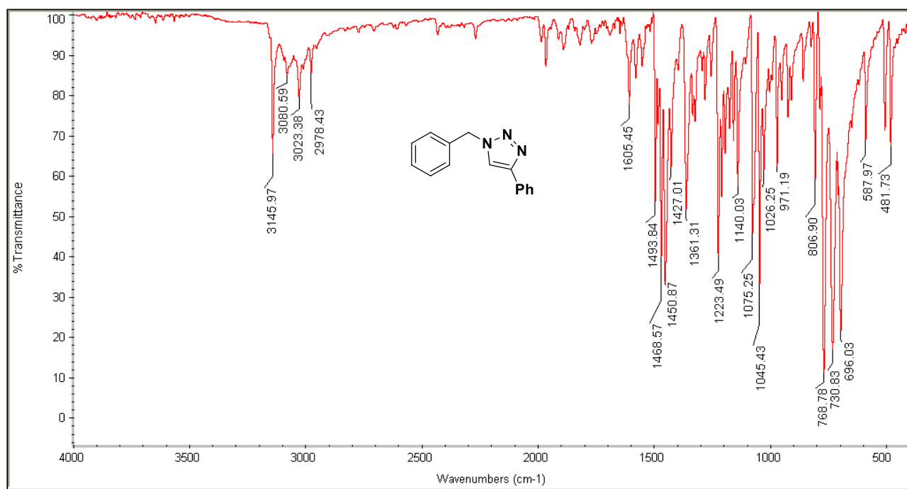
Fig. S3 FT-IR of 1-Benzyl-4-phenyl-1H-1,2,3-triazole ( 5a , 5b and 5c , Table 3, Entries 1-3)
