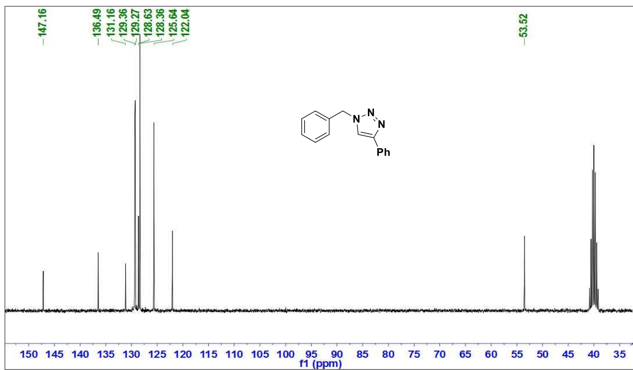
Fig. S5 ^{13}\text{C} -NMR of 1-Benzyl-4-phenyl-1H-1,2,3-triazole ( 5a , 5b and 5c , Table 3, Entries 1-3)
