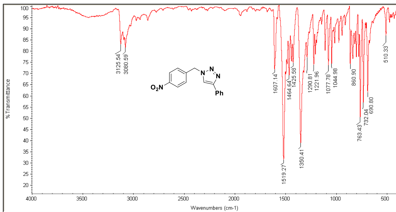
Fig. S8 FT-IR of 1-(4-nitrobenzyl)-4-phenyl-1H-1,2,3-triazole ( 5f , Table 3, Entry 6)
